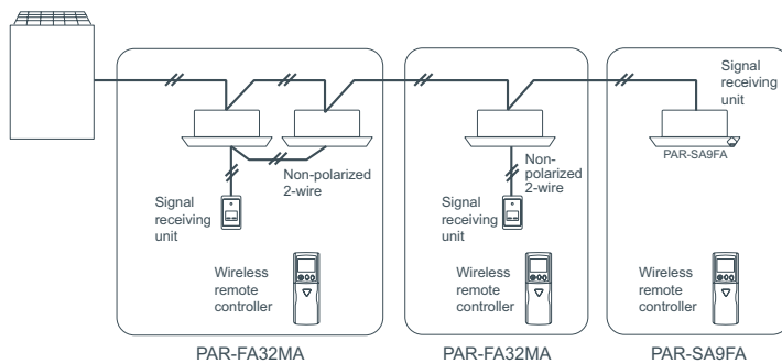
PAR-SA9FA (4-way Cassette signal receiver)
